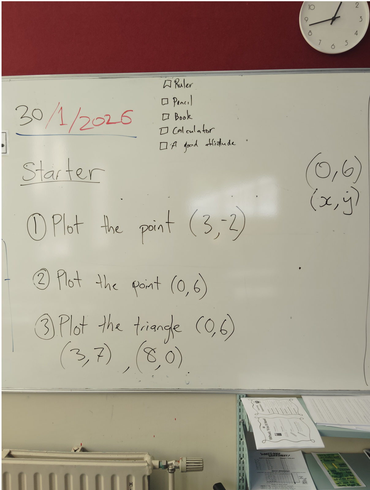
Figure 1: Simple example of points on a Cartesian plane
